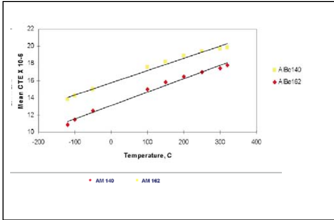
The graph depicts the Coefficient of Thermal Expansion for AlBe alloys.
